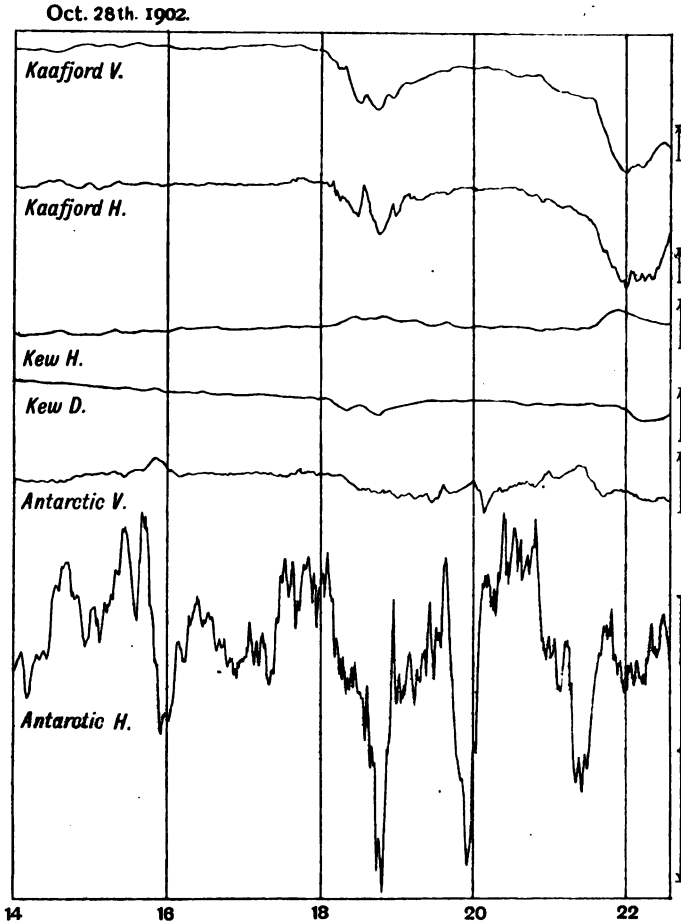
FIG. 28.—ARCTIC-KEW-ANTARCTIC CURVES.
